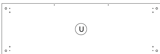
FS2838 1320x436x38mm
